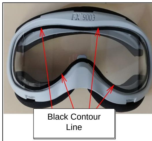
Fig. 23 - FX® 9003 Goggle Assembly (Double lens with open cell configuration)
